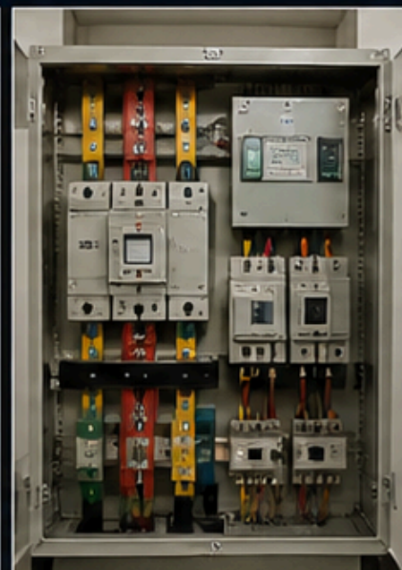
ELDP PANEL
