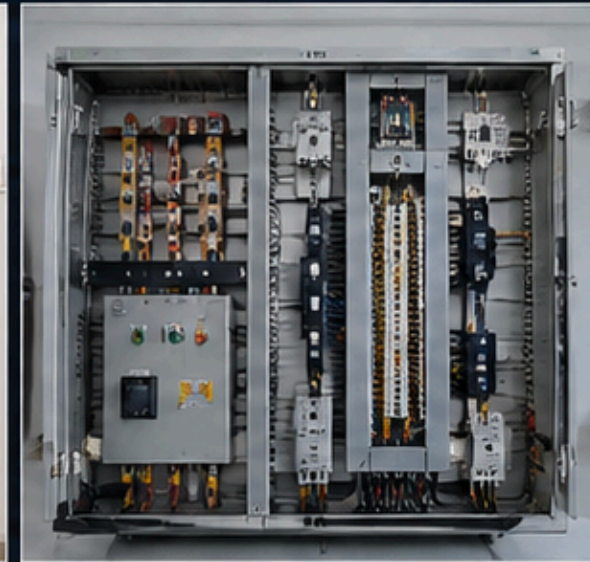
PDB PANEL
